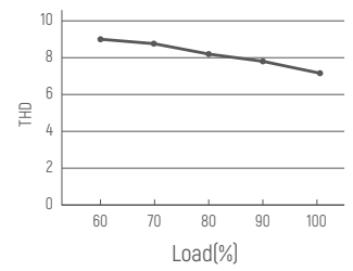
THD vs Load
