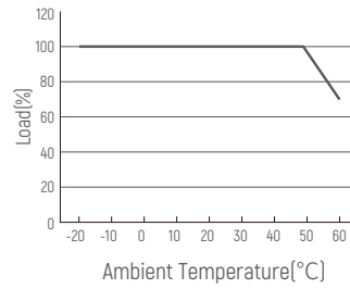
Derating Curve
