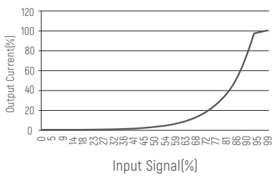
Dimming Curve
