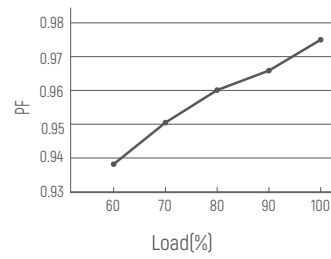
PF vs Load
